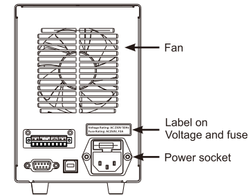
Diagram of Rear Panel
